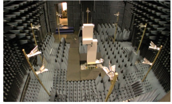
Figure 2. Setup used in the MIMO OTA testing.
