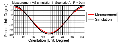
Figure 8. Simulation and measurement comparisons for single plane wave with AoA = 0 degrees in terms of phase variations at radius = 9cm
