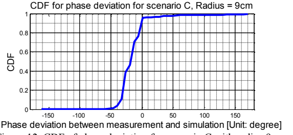
Figure 12. CDF of phase deviation for scenario C with radius 9cm.
