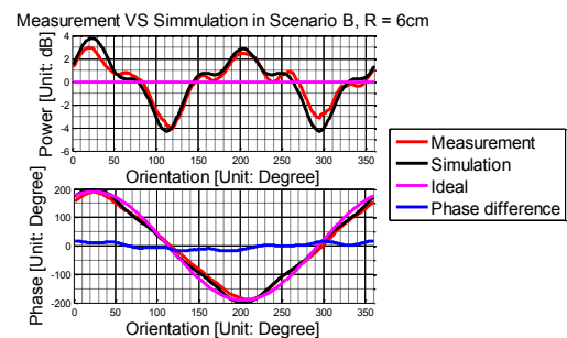
Figure 9. Simulation and measurement comparisons for single plane wave with AoA = 22.5 degrees in terms of power and phase variations
