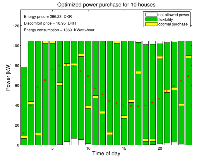
Fig. 2. Optimized power purchase for ten houses. Yellow is predicted optimized energy purchase, green is flexibility and red is power if the room temperature is kept constant.
