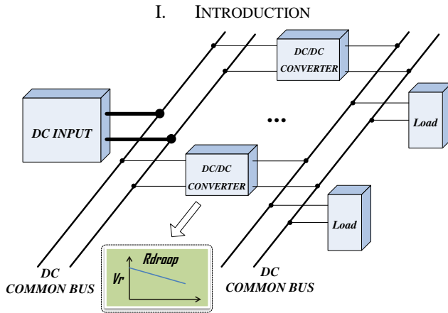
Figure 1. Droop-controlled paralleled dc-dc converter system
