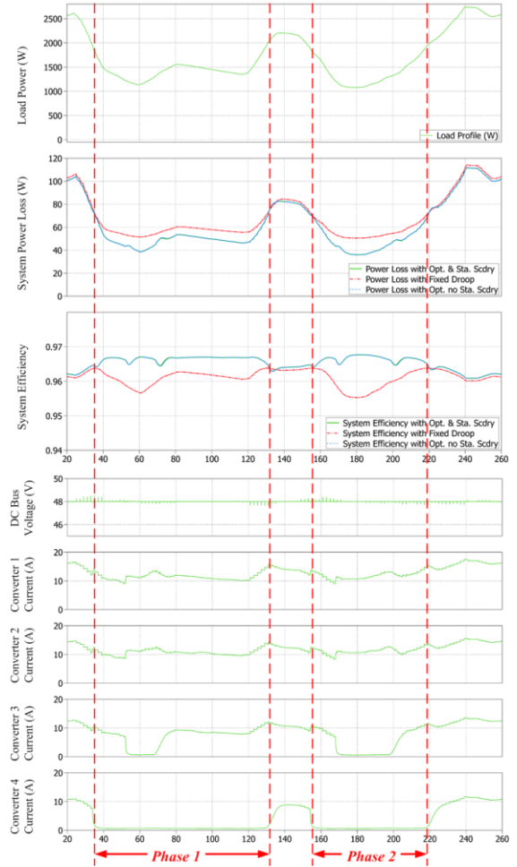
Figure 14. Simulation Results with Random Load Profile
