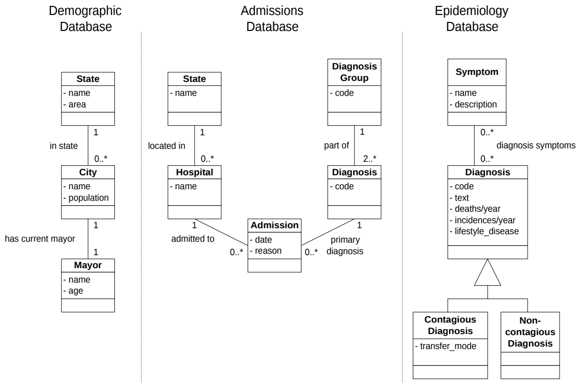
Figure 1: UML Schema of Case Study
