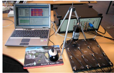
Figure 7. Measurement setup.
