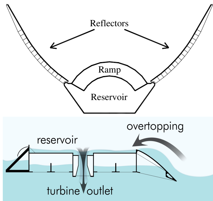
Fig. 1. Above: Main components of the WD. Below: The basic principle of the WD, 1) waves overtopping a ramp, 2) water stored in a reservoir above sea level and 3) water discharged through hydro turbines.
