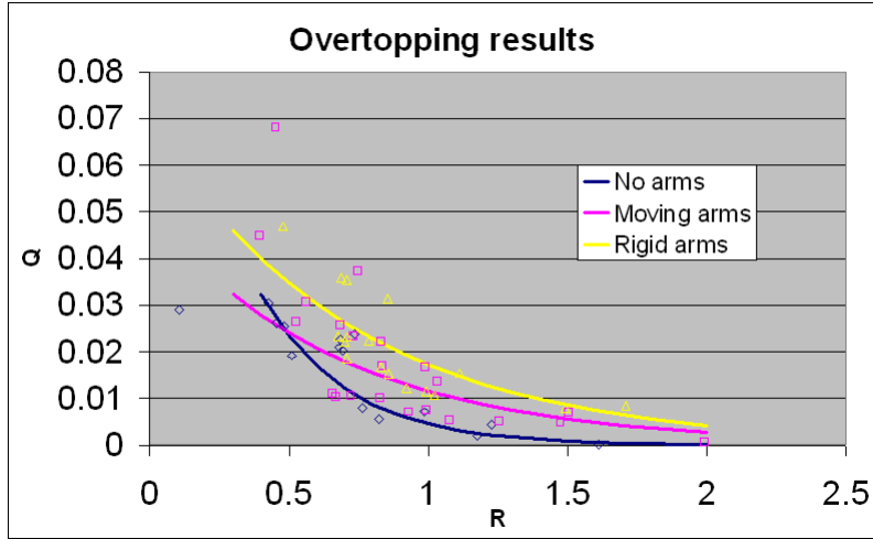
Figure 6: Overtopping results
