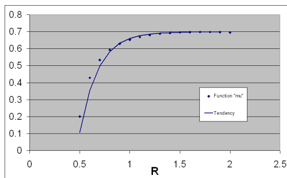
Figure 8: Estimation of the function \mu
