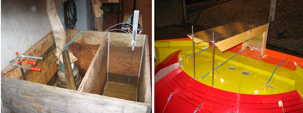
(a) Interim tank, with pump and wave gauge (b) View of the Wave Dragon tank, with exhausting holes and reflecting plates
