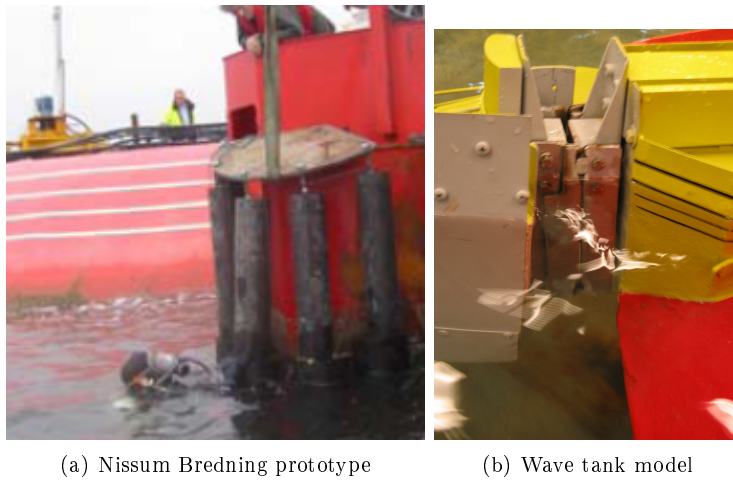
Figure 2: Rubber fender and equivalent setup (metal plates)
