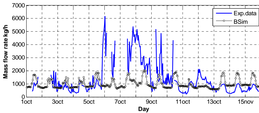
Figure 4. Mass flow rate in the DSF cavity measured with the tracer gas method and simulated in BSim.
