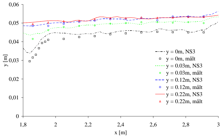
Figure 7 Comparisons of length profiles of water surfaces parallel to overflow crest upstream crest in side weir, y is horizontal distance from crest, NS3 is computed and "mält" is measured.
