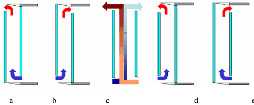
Figure 1. AIF flow path: EA-a); SA-b); RAF-c); OAC-d); IAC-e) [Annex 44 (2005)]
