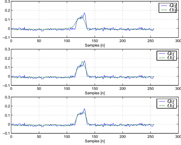
Fig. 2. Illustration of the Karhunen-Loève approximation of \alpha_f which contain a typical scratch. The first approximation is based on the one most approximating coefficient, the second approximation is based on the five most most approximating coefficients, and the third approximation on the seven most approximating coefficient.
