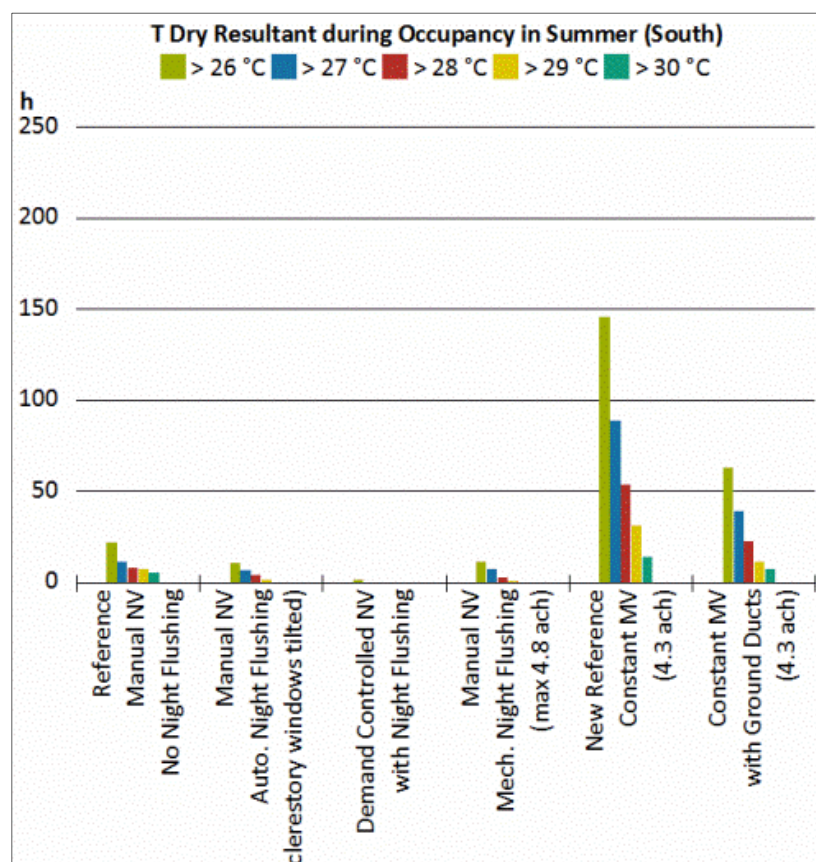
Figure 9: Frequency of dry resultant temperature overshooting in summer with night flushing systems and ventilation through ground ducts
