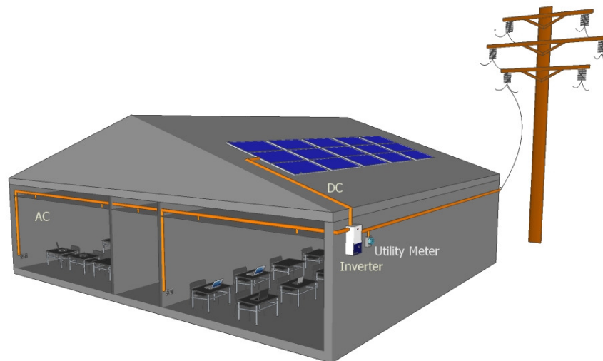
Figure 11: Grid connected PV-system
