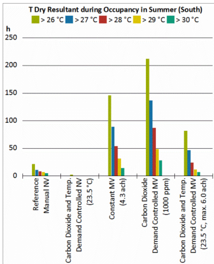
Figure 7: Frequency of dry resultant temperature overshooting in summer with different ventilation systems
