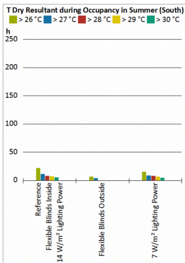
Figure 8: Frequency of dry resultant temperature overshooting in summer with different measures reducing gains
