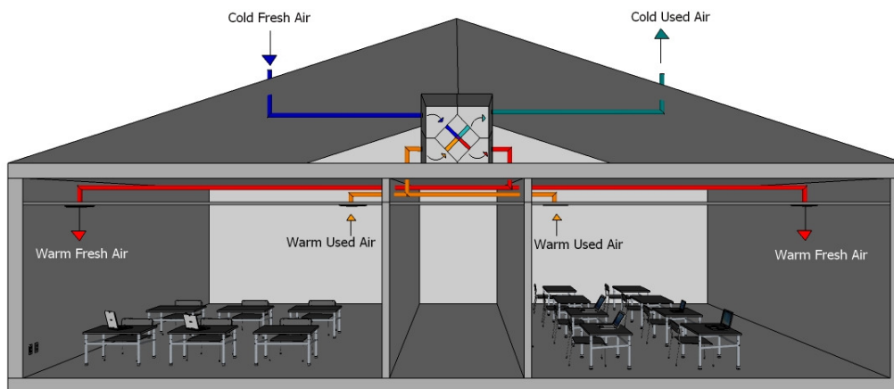
Figure 9: Schematic of MVHR-system.
