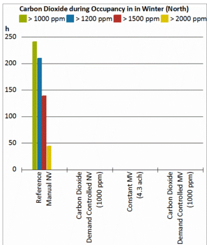
Figure 5: Frequency of carbon dioxide overshooting in winter with different ventilation systems
