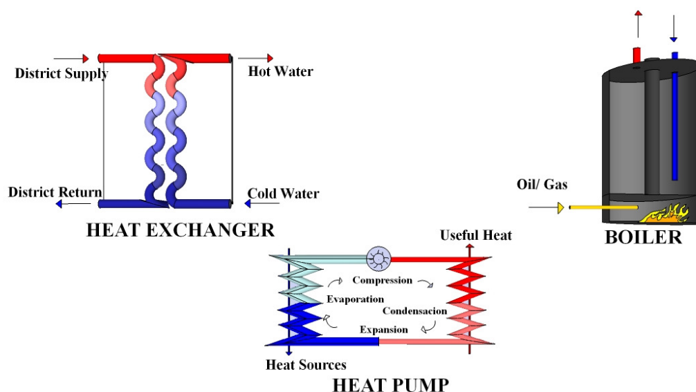
Figure 13: Three different types of heating supply systems
