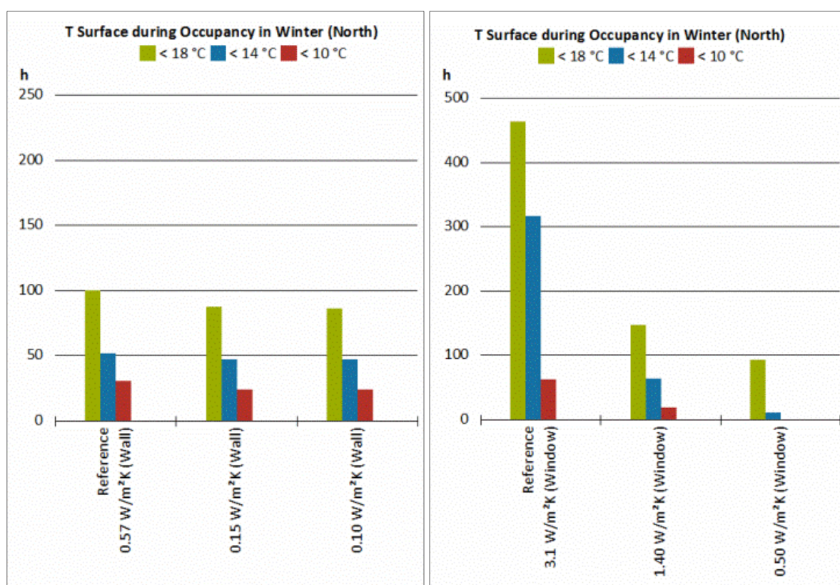
Figure 1: Frequency of surface temperature undershooting at the outer wall and windows with different insulation standards
