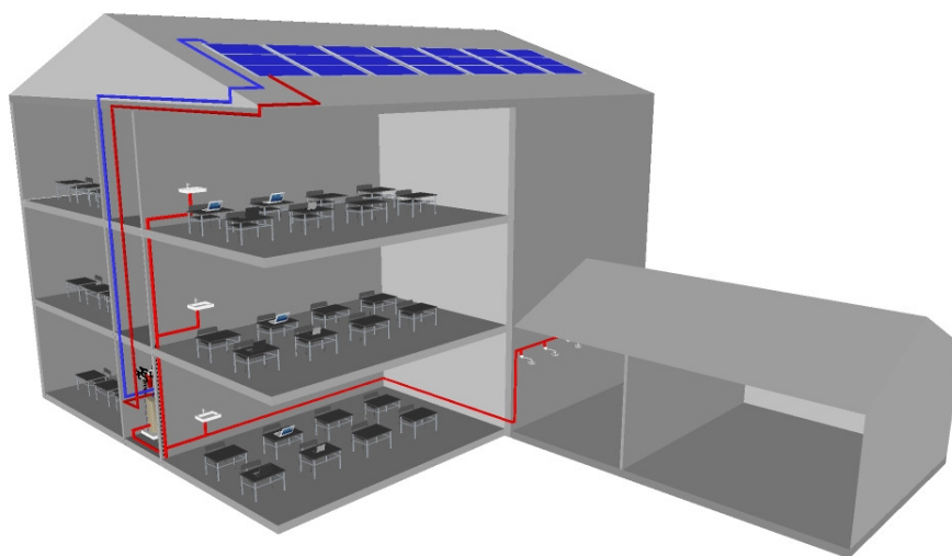
Figure 12: Thermal solar system for heating of hot water
