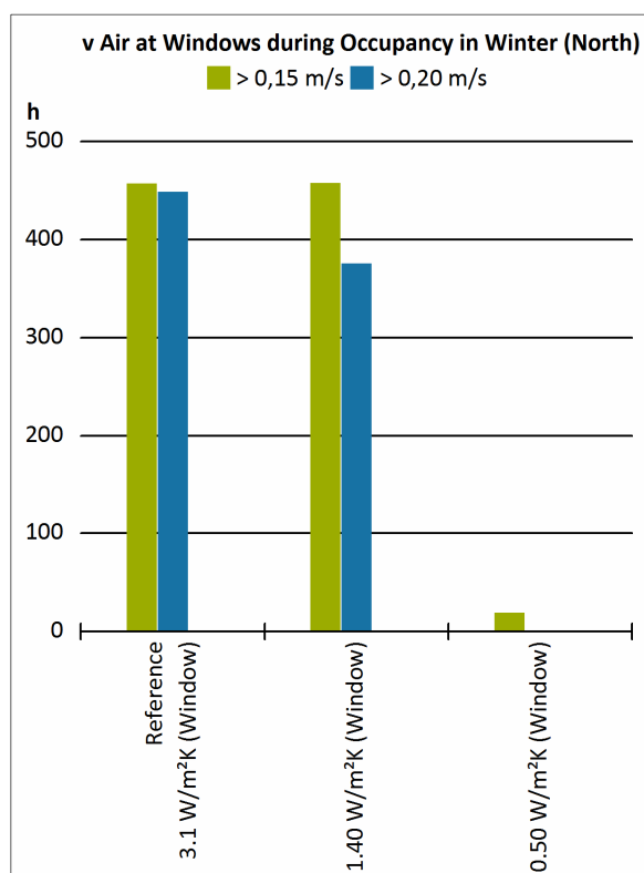
Figure 2: Frequency of down draught near the windows with different insulation standards
