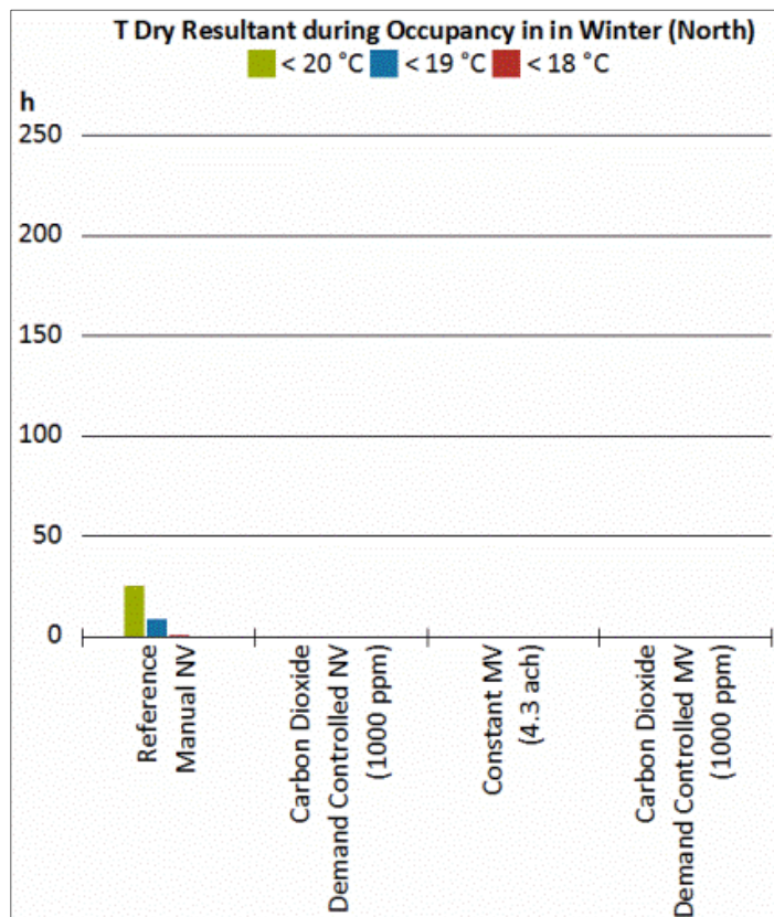
Figure 6: Frequency of dry resultant temperature undershooting in winter with different ventilation systems
