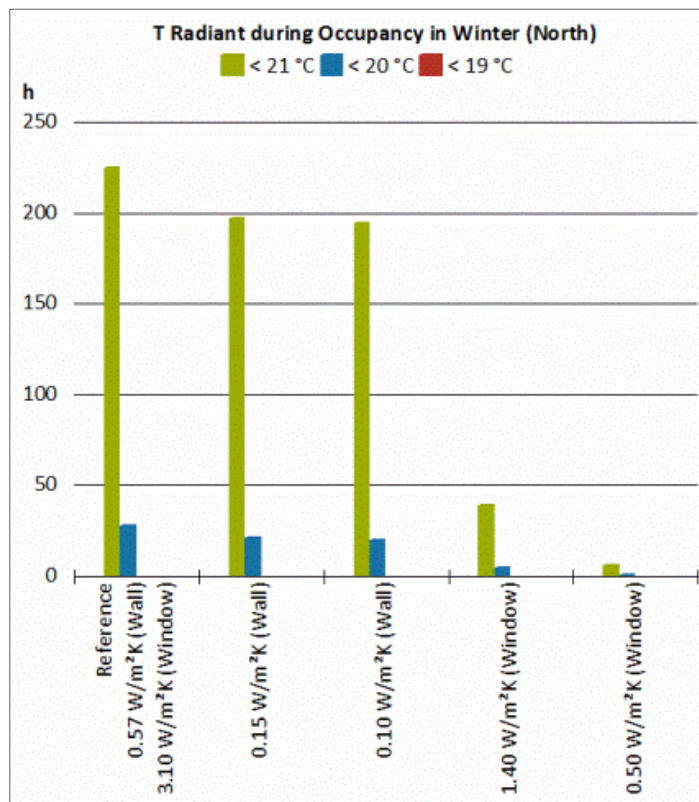
Figure 3: Frequency of mean radiant temperature undershooting with different insulation standards at the outer wall and windows
