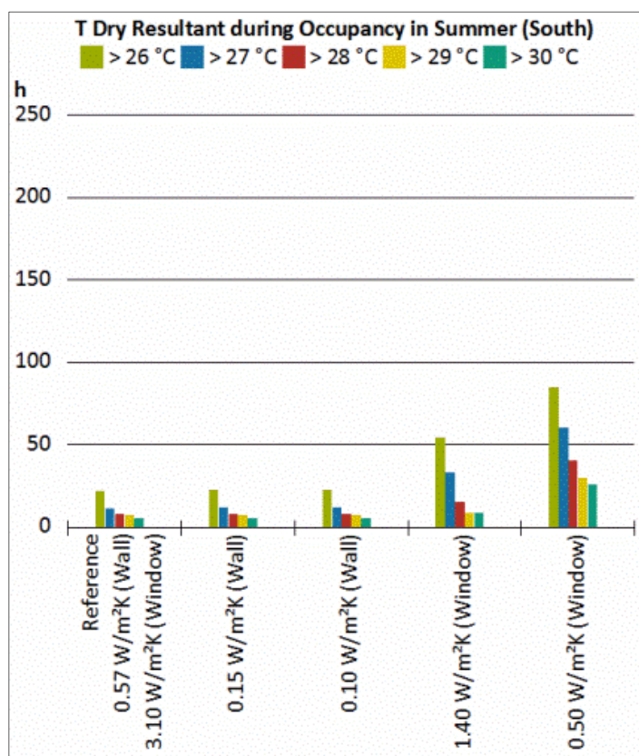
Figure 4: Frequency of dry resultant temperature overshooting with different insulation standards at the outer wall and windows
