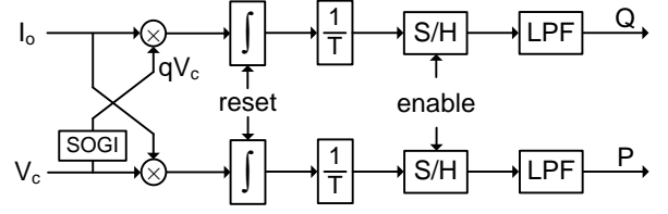
Fig. 3. Real and reactive power calculation where I_o is the output current and V_c is the voltage across the capacitor. The period T depends on the droop frequency \omega . A second-order generalized integrator (SOGI) was used to generate the quadrature voltage component. The real and reactive power calculations were sampled via a sample and hold (S/H) and filtered via a low pass filter (LPF).
