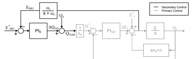
Fig. 8. Block diagram of the secondary amplitude restoration cascaded with the reactive power sharing loop where PI_E and PI_{QS} are the PI compensators for the voltage restoration and reactive power sharing respectively.
