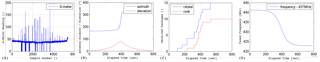
Fig. 3. Plot of the raw data recorded during a single satellite pass of 10 minutes: (A) shows the plot of the raw signal strength measurement per sample, (B) shows the antenna azimuth and elevation, (C) shows the amount of overall received packets and how many passed the CRC check, and (D) shows the change in carrier frequency as a consequence of the Doppler shift effect [12]
