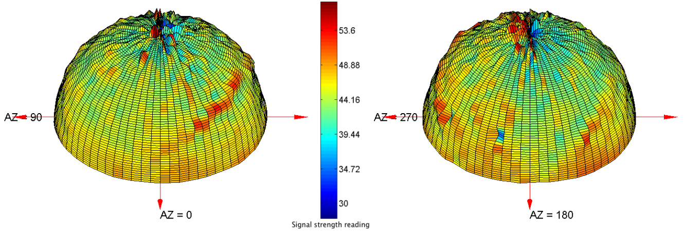
Fig. 8. Two 3D background noise plots (noise maps) calculated from 2500 passes covering the full 360° hemisphere around the Aalborg ground station. Azimuth resolution: 5° Elevation resolution: 1°
