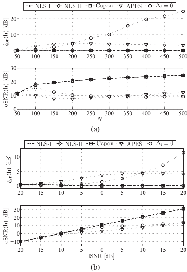
Fig. 2. Performance measures of synthetic signal as a function of (a) N and (b) iSNR.
