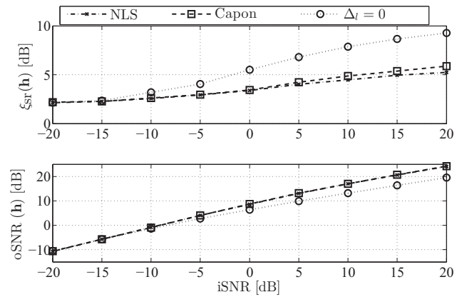
Fig. 3. Performance measures of speech signal as a function of iSNR.
