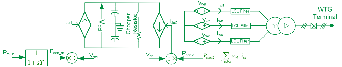
Fig. 2 Simplified model of a wind turbine generator with full scale converter (WTG-FSC)
