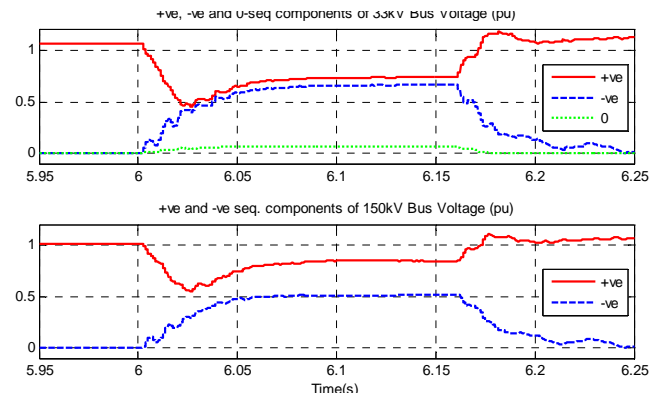
Fig. 12 Sequence components of the voltages in the 33kV and 150 kV grid during the L-G fault.
