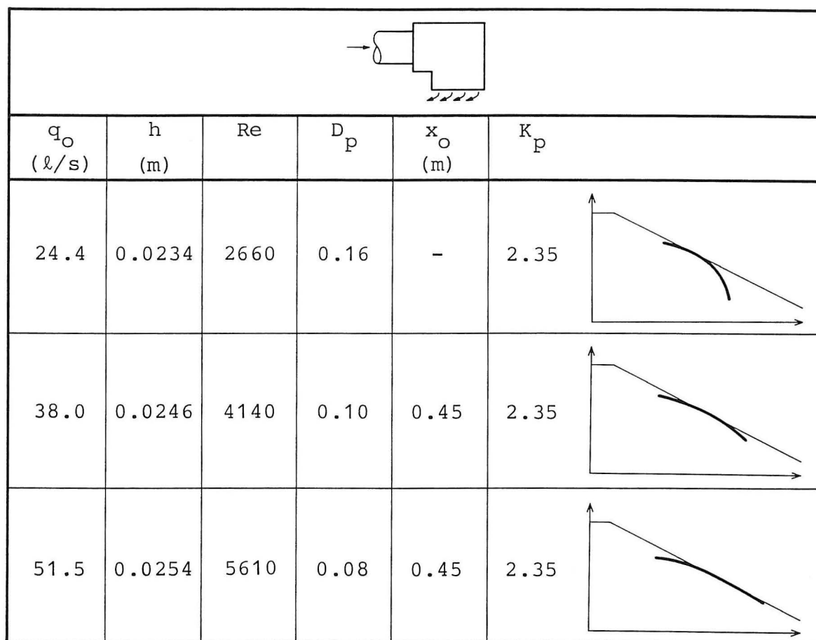
Fig. 4. Measurements of the isothermal wall jet from a slot diffuser with small width, \ell = 0.6 m. The diffuser is adjusted for a single horizontal wall jet.
