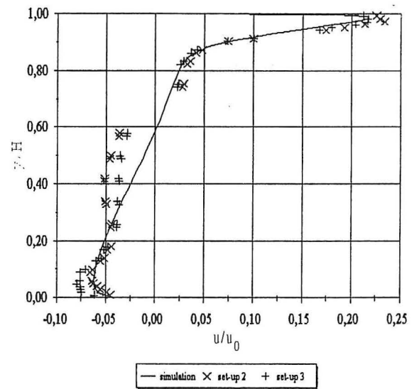
Velocity profiles in set-up 2 and 3
