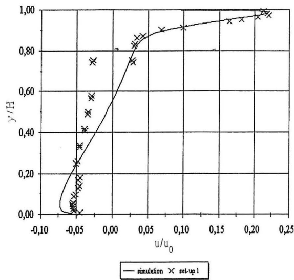
Velocity profiles in set-up 1
