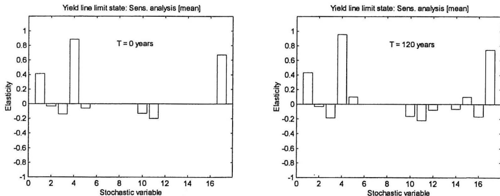
Figure 4 : Sensitivity analysis for yield line limit state at t = 0 years and at t = 120 years.
