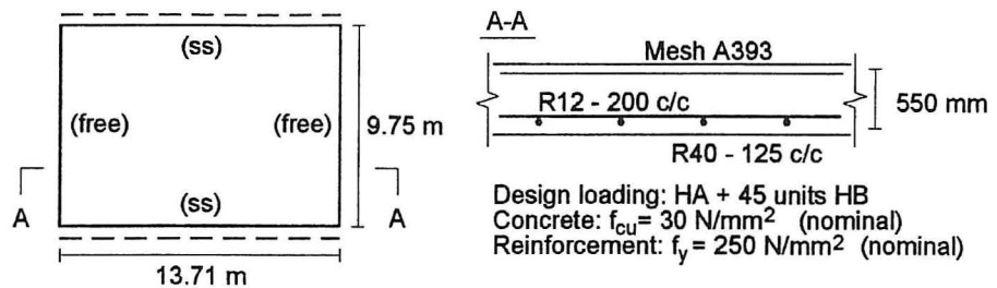
Figure 1. Bridge data.
