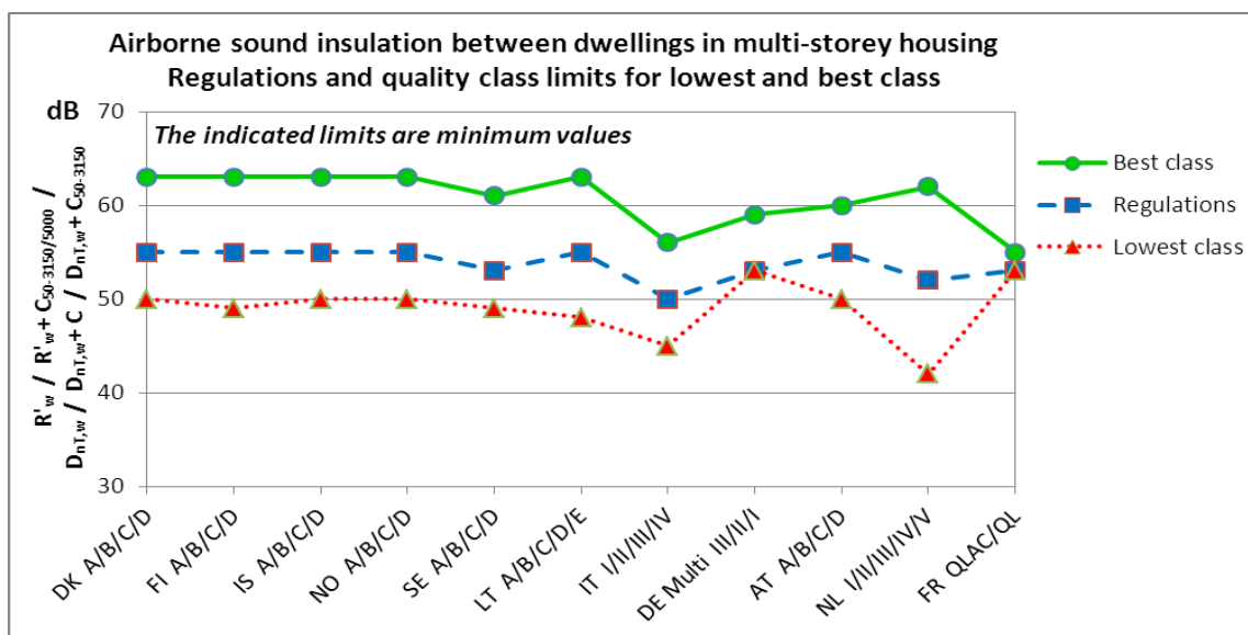
Figure 2: Airborne sound insulation limits for highest and lowest classes in 11 classification schemes in Europe and regulatory requirements for the same countries. Data are from [13, 19]. Note: The graphs present the numbers only. No conversions between descriptors have been applied.
