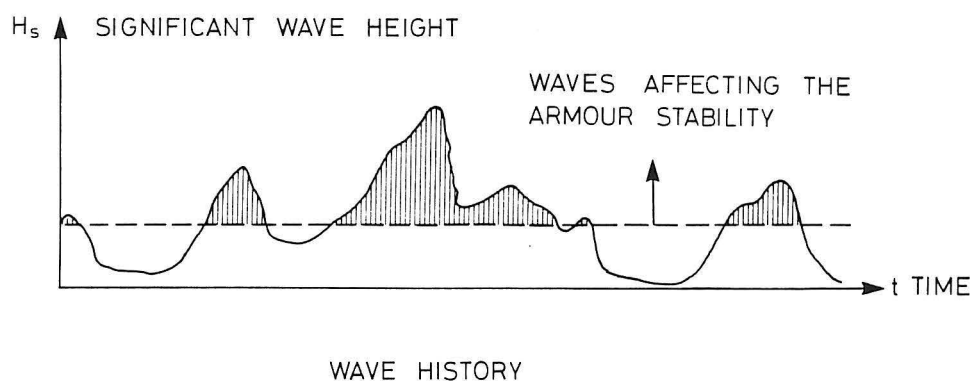
Fig. 14. Wave history.
