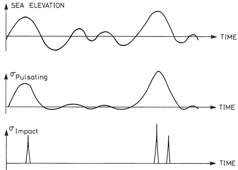
Fig. 15. Realization of wave induced stresses in an armour unit.
