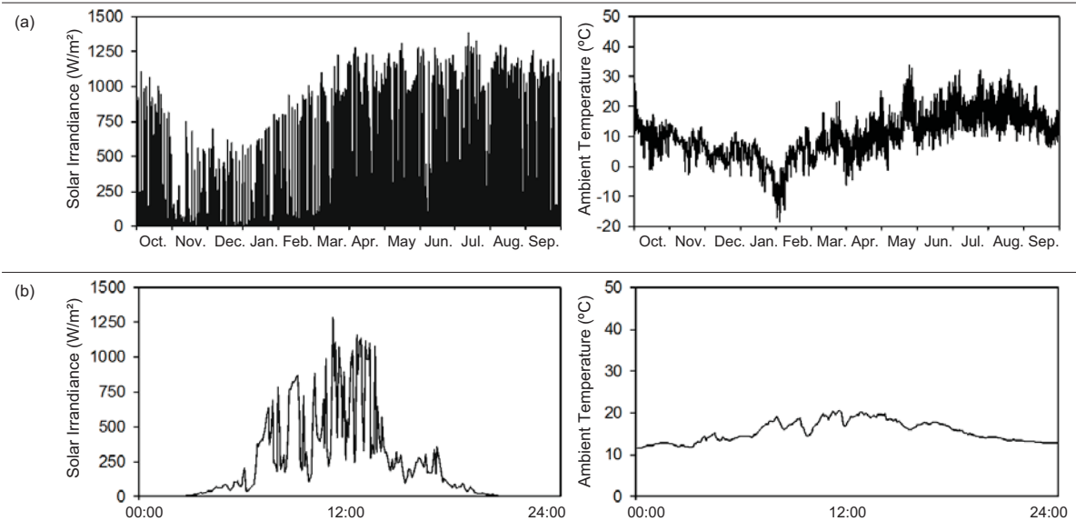
Fig. 7: Mission profiles from recorded data (5 minutes per sampling data) at Aalborg University: (a) yearly profiles from October 2011 to September 2012 and (b) a daily mission profile (cloudy day).
