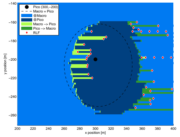
Fig. 8: Profile Set 1, UE speed 60 km/h, cells fully loaded.
