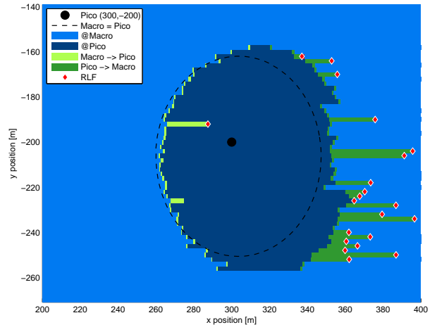
Fig. 9: Profile Set 2, UE speed 60 km/h, cells fully loaded.
