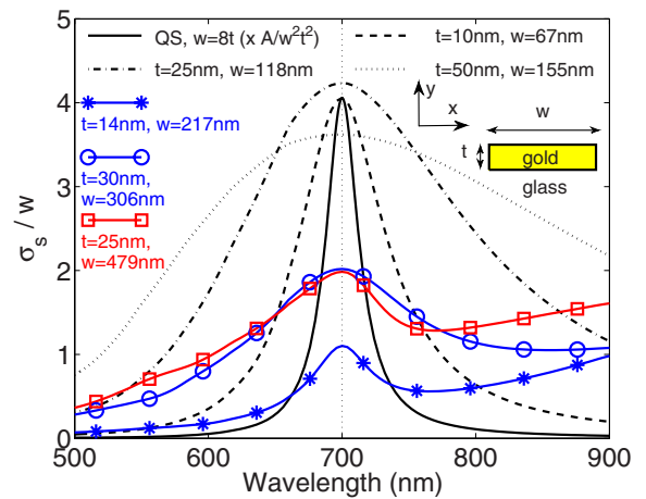
FIG. 1. (Color online) Scattering cross section vs wavelength for a plane p -polarized wave incident on a gold nano-strip of thickness t and width w embedded in glass. For w=67 –155 and 479 nm, and the quasistatic (QS) case, the incident wave propagates along the y axis. For w=217 and 306 nm, the incident wave propagates at 45^\circ relative to the x axis.
