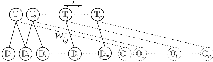
Fig. 2. Example of the bipartite graph that must be solved for each frame. Each tracker T_i is connected to all detections D_j that lie within its search radius and to one occlusion node O_i .
