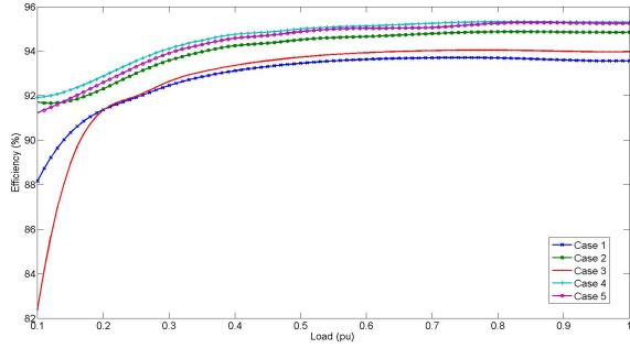
Fig. 19. Efficiency comparison
