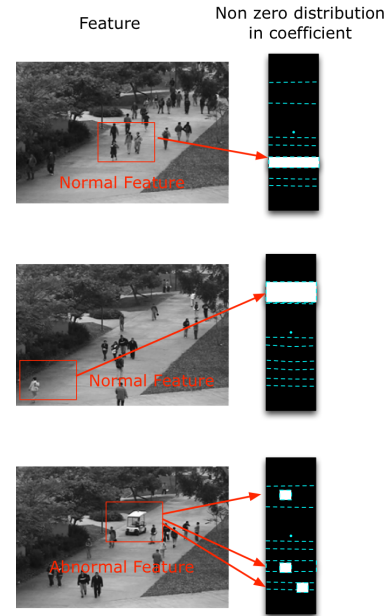
Fig. 1. Ideal structured sparsity in normal and abnormal features. As normal features, their non zeros in coefficients should only distributed in the atoms with the same behavior; as abnormal features, their non zeros in coefficients should spread over atoms.
