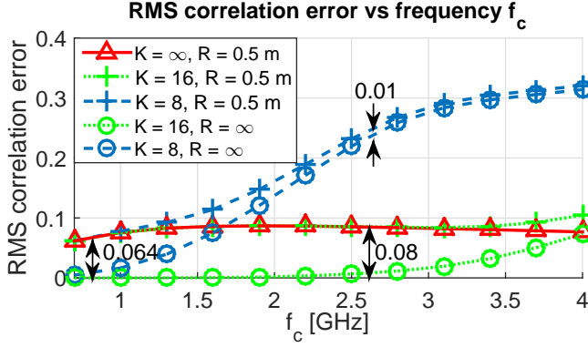
Fig. 5. RMS error for the SCME Urban micro channel model as a function of carrier frequency. Deviation between ideal and small setups are marked at 751 MHz and 2655 MHz.
