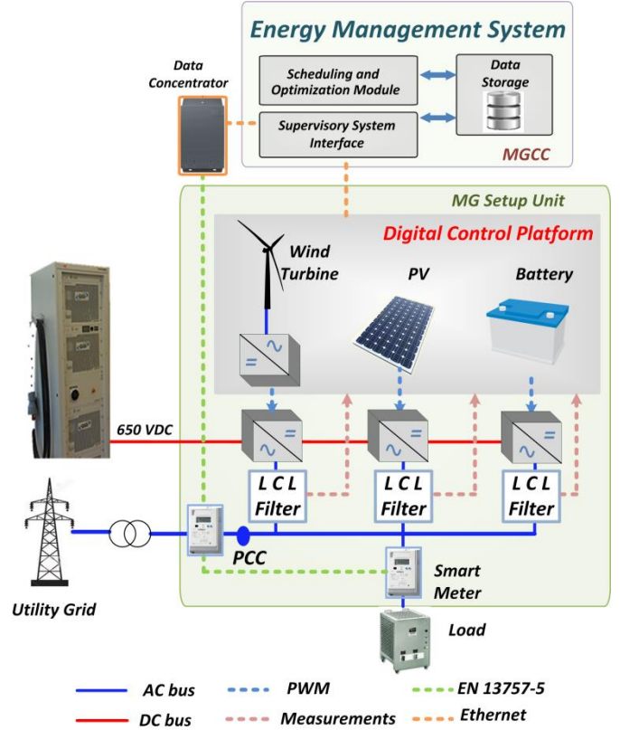
Fig. 13. Energy management study case and implementation.
