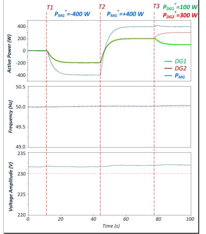
Fig. 12. Tertiary control of power flow.
