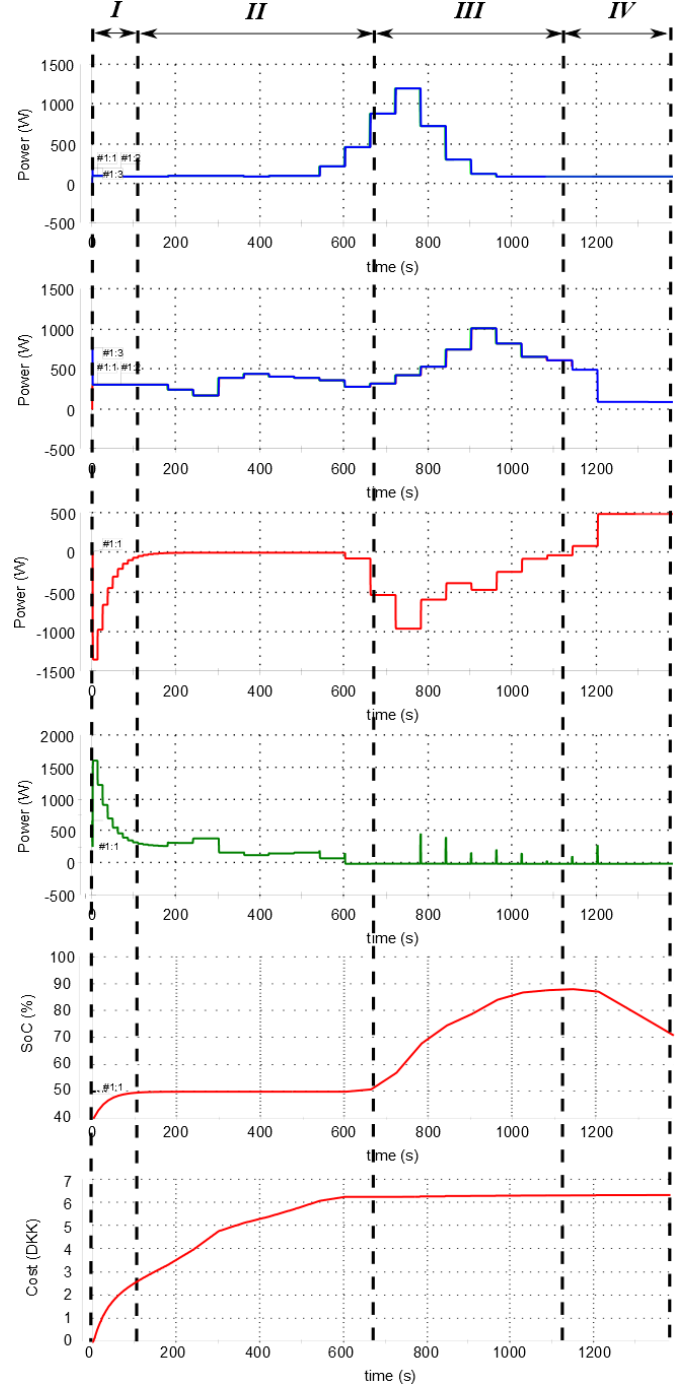
Fig. 15. Results obtained using EMS. Top to bottom: PV power, WT power, battery power, power absorbed from the main grid, SoC of the battery
