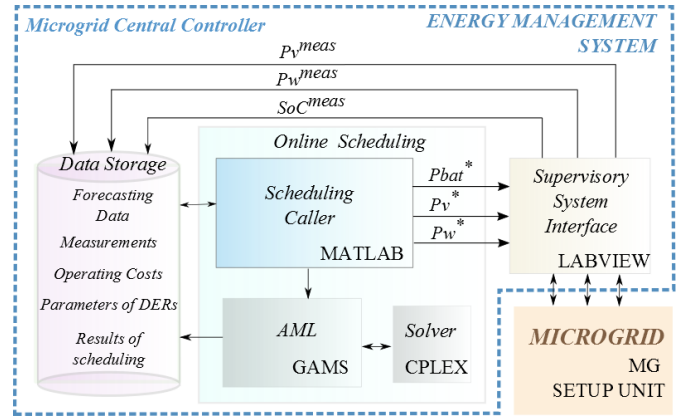
Fig. 14. Data flow in the EMS.
