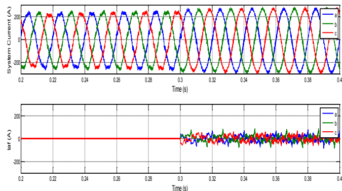
Fig. 5. System and Active power filter current
