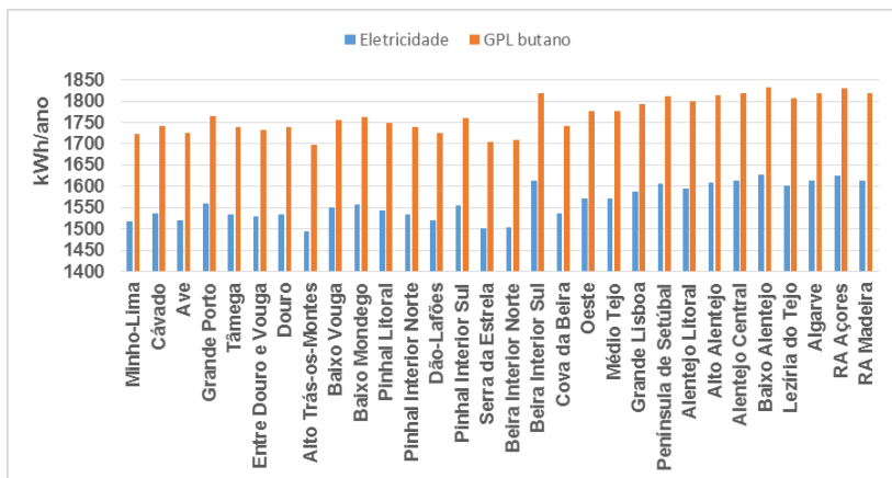
Fig. 2. Potencial de anual energy consumption reduction.
