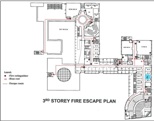
Figure 5-9 Building C's Floor Plan – 3
