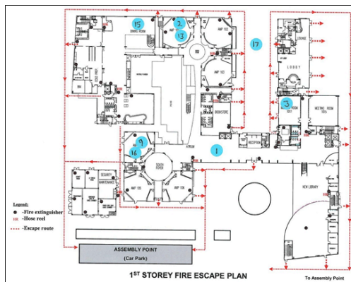
Figure 5-7 Building C's Floor Plan – 1
