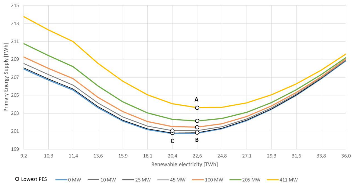
Figure 3. Primary energy supply (PES) in 2020 energy system with different electrolyser capacities and renewable electricity capacities
