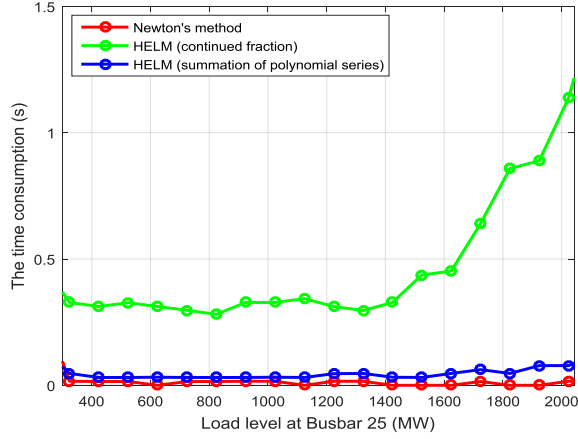
Figure 11. Comparisons of the time consumptions for (i). Summation of the power series; (ii). Continued fraction and (iii). Newton-Raphson method.
