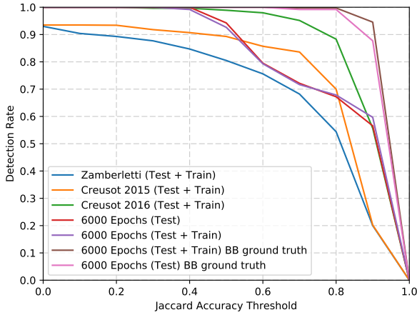
Figure 3: Test results on the Arte-Lab dataset.
