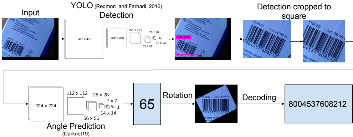
Figure 1: Overview of our system.
