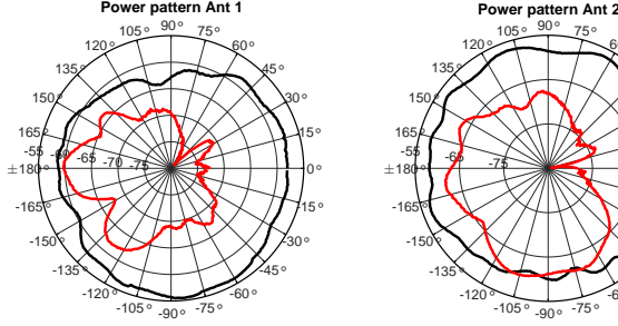
Figure 8. The measured total gain patterns of the two antennas on the second mockup in the free space and user influence mode.
