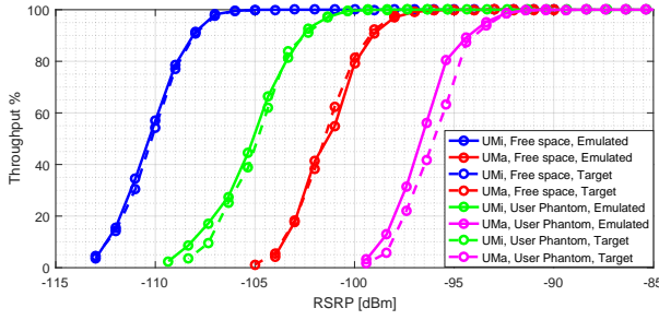
Figure 15. The measured throughput results under the target and emulated (with K = 8 ) channel models for the first LTE mockup in the free space mode and user influence mode.
