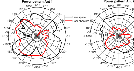
Figure 7. The measured total gain patterns of the two antennas on the first mockup in the free space and user influence mode. The radial axis in the polar plot denotes the measured total gain in dB.
