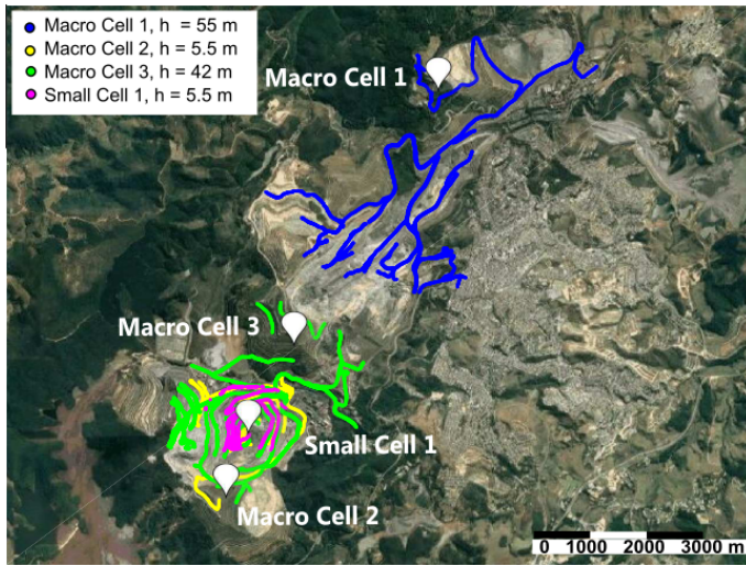
Figure 1. Measurement routes and transmitter positions in Mine 1. The height above ground level, h , is also displayed in the legend.
