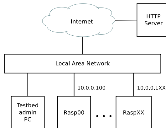
Figure 1. Testbed setup.
