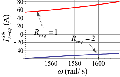
Fig. 6. Relationship of I_{n-og}^{5th} and \omega with fixed R_{virq} (conventional ACSC).
