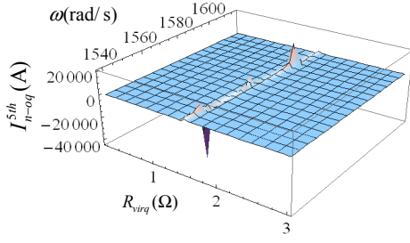
Fig. 5. Relationship of R_{virq} , I_{oq}^{5th} and \omega (conventional ACSC).
