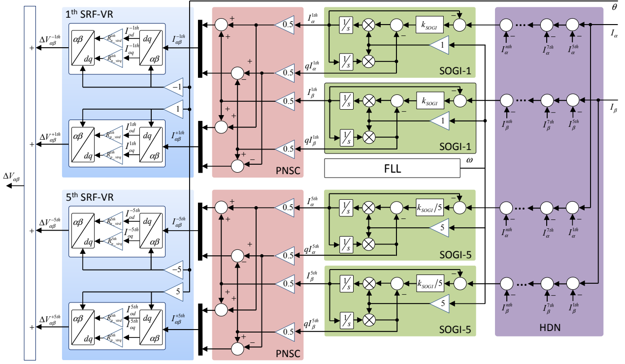
Fig. 8. Overview of the proposed control scheme.
