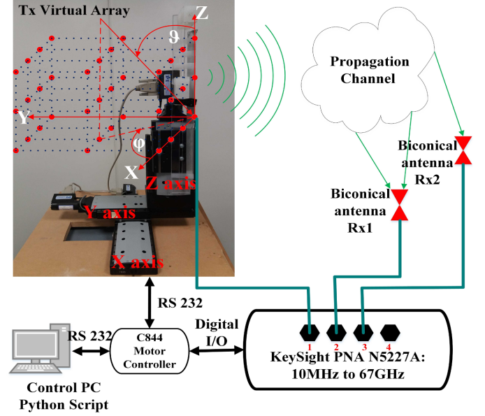
Fig. 1: Measurement Setup.
