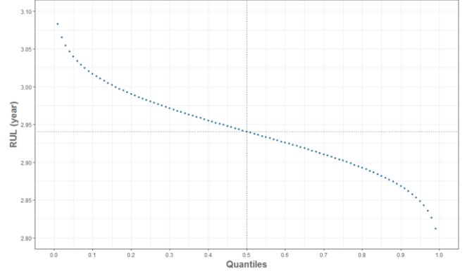
Figure 6. Uncertainty in RUL prediction at year 15 for the component shown in Figure 5
