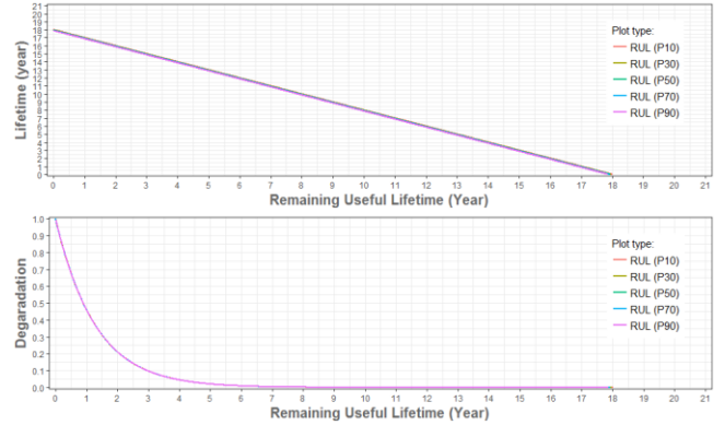
Figure 7. Remaining useful lifetime of a component plotted against its lifetime and degradation level
