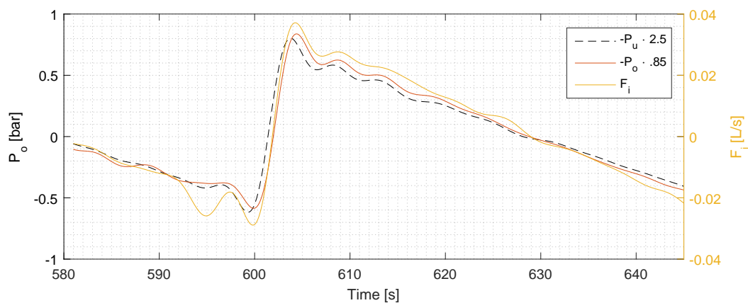
Figure 4. Comparison of F_i , P_u , and P_o .
