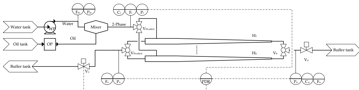
Figure 1. Sketched diagram of the plant, including the feeding system, the hydrocyclone array, and the transmitters used in the study. C_i , C_u : Turner Design TD-4100XDC (TD-4100) fluorescence monitors; F_{in} , F_i , F_u : electromagnetic flow transmitters; F_o : Coriolis flow transmitter; OP: oil pump; P: pressure transmitter; PDR: pressure drop ratio; V: valve; WP: water pump.
