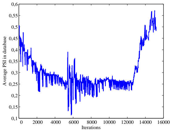
Figure 8: The development of the average value of all PSI in the database after each iteration (each look up in the database). Initially PSI is around 0.5 and the game is played by an unskilled player. The player slowly improves his skills and the average value of PSI increases correspondingly.
