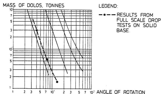
EXAMPLES OF ISO-STRESS GRAPHS FOR ROCKING UNREINFORCED DOLOSSE OF IDENTICAL CONCRETE. WAIST RATIOS 0.30-0.36
