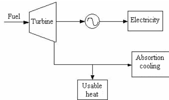
Figure 5-2: Trigeneration with absorption chiller
