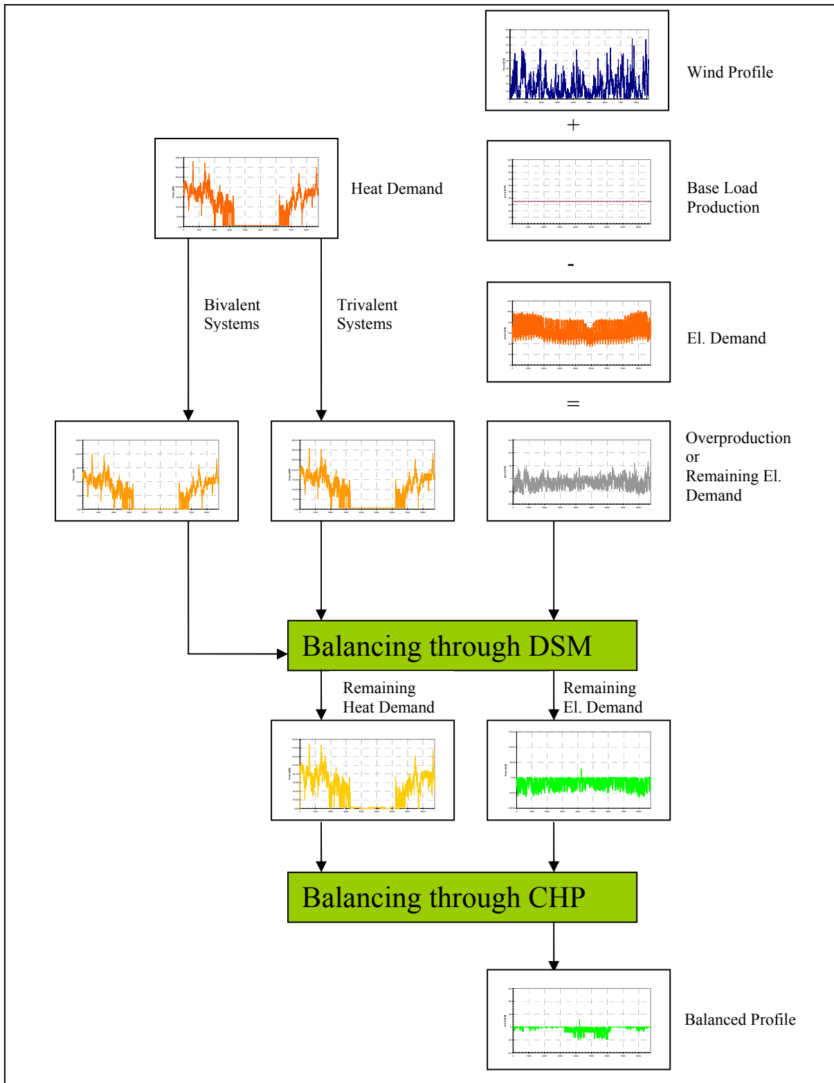
Figure 3-17: Schematic structure of the calculations
