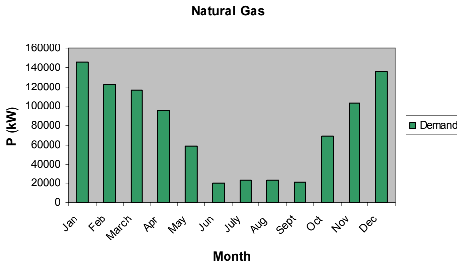
Figure 5-27: Monthly natural gas demand (Trigeneration system)
