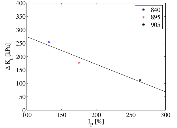
Figure 13: \Delta K_t as a function of I_P .
