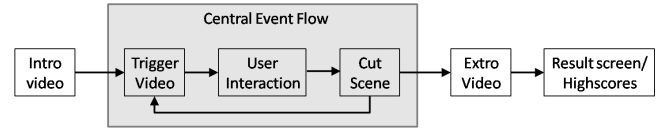
Figure 8: Overview of general game flow with central interaction sequence highlighted.
