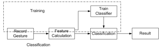
Figure 3: The standard classification pipeline has been integrated in MoGLE.
