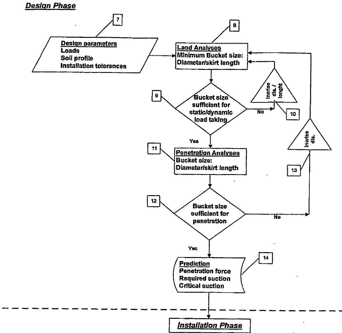
Figure 2. The design Phase
