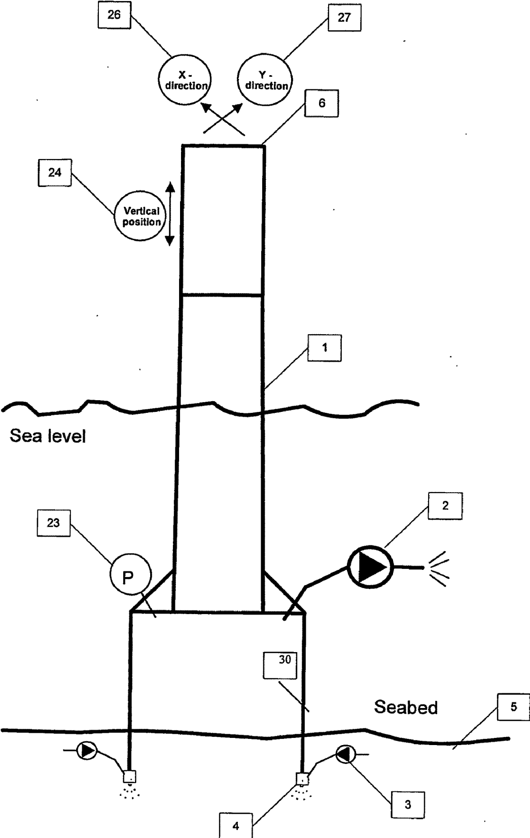
Figure 1. The foundation structure
