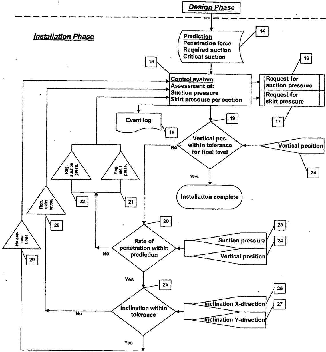
Figure 3. The Installation Phase
