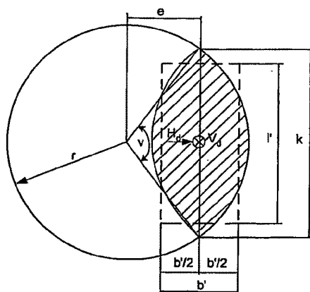
Figure 10. Principle to determine effective area.
