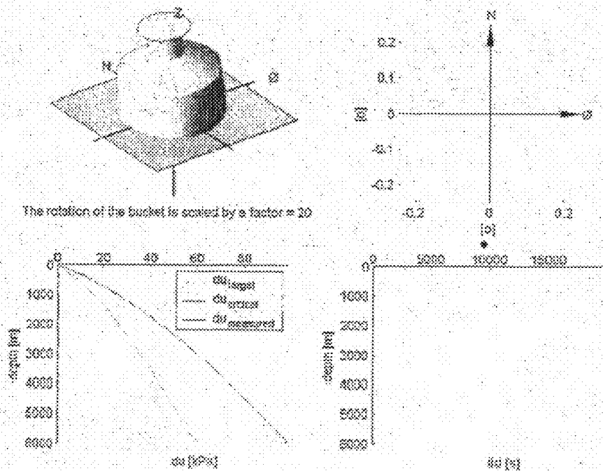
Figure 12. Presentation of operation and control data
