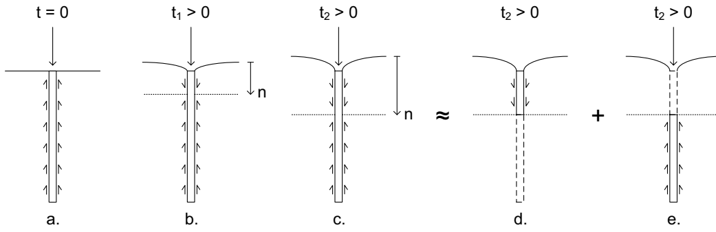
Figure 3: Simplification of the mechanisms for an axially loaded pile in a swelling soil. n is the height of the swelling zone. t_1 < t_2 .
