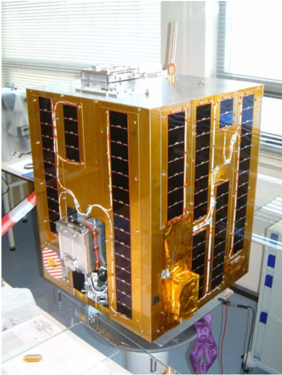
Caption: Figure 2. The SSETI-Express flight mode
