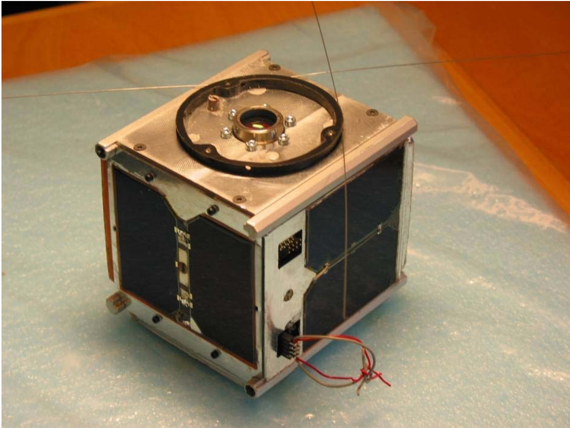
Caption: Figure 1. The AAU CubeSat flight model.
